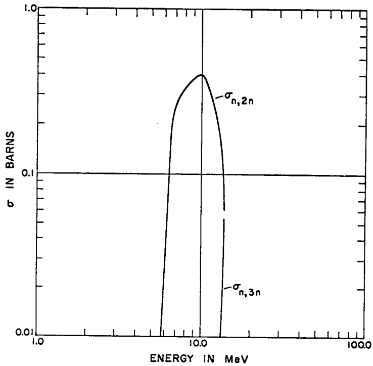
Fig. 17. \sigma_{n,2n} and \sigma_{n,3n} for ^{240}\text{Pu} .
